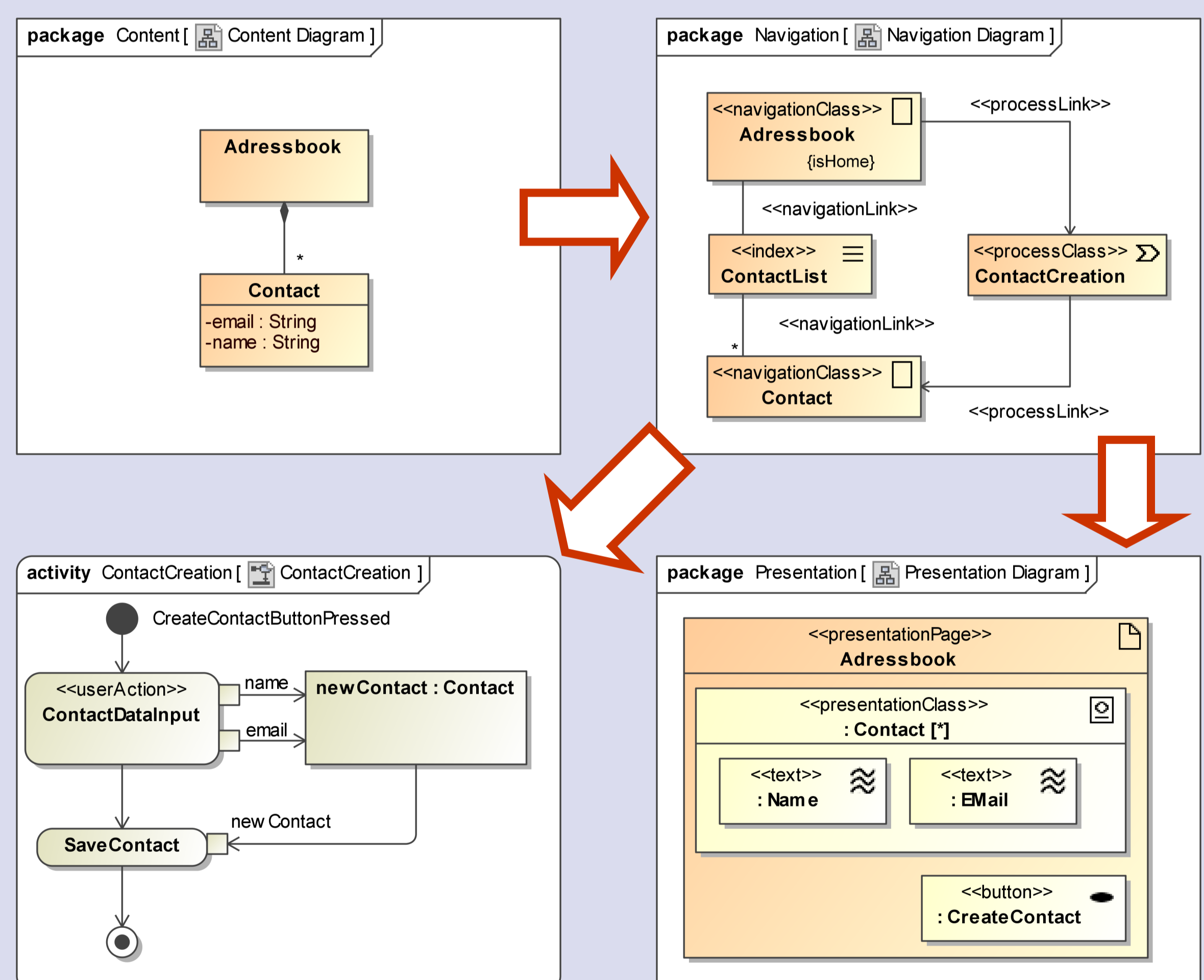
Modeling with MagicUWE: Address book example
